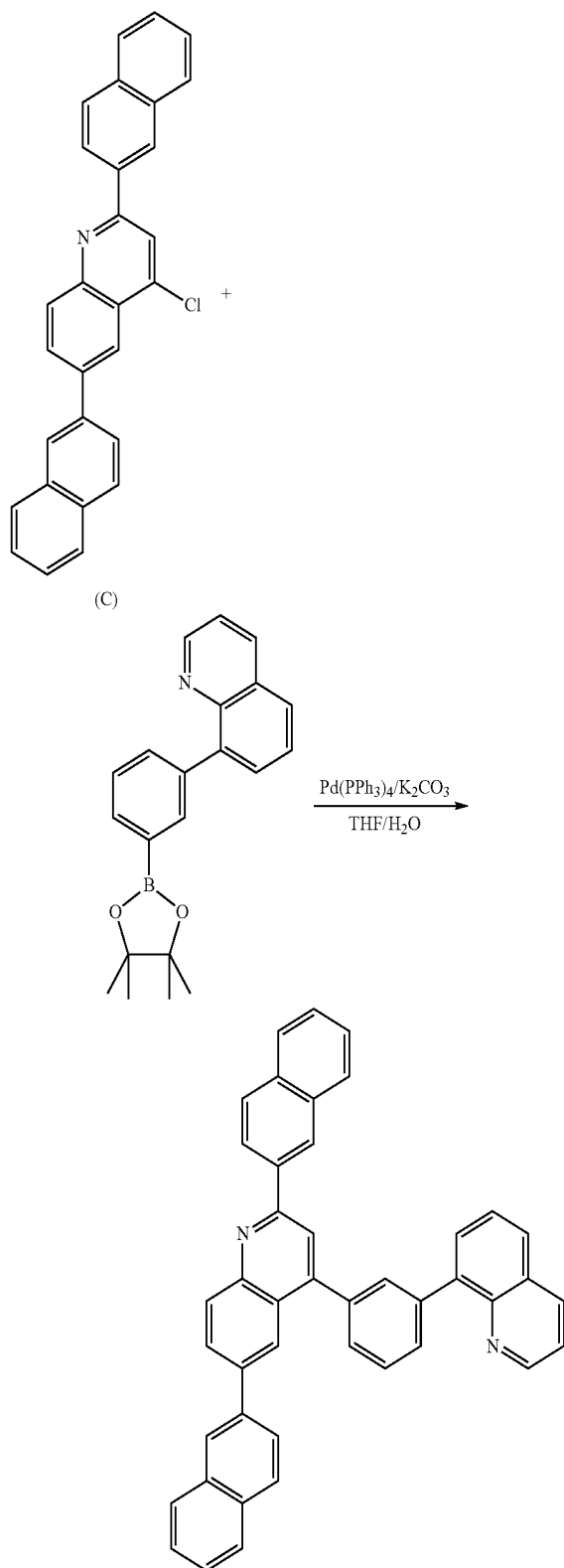
[Reaction Scheme 7]
