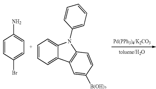
[Reaction Scheme 9]
