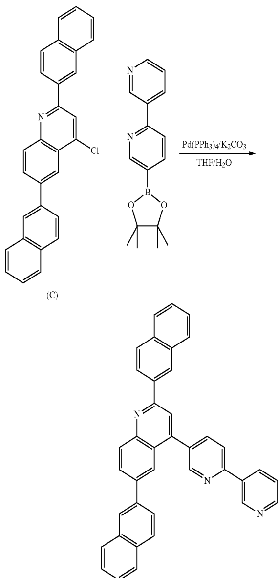
[Reaction Scheme 4]
