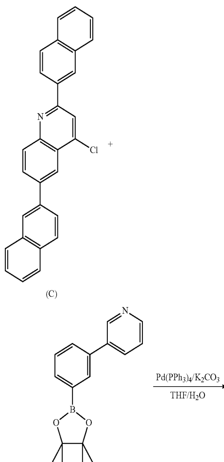
[Reaction Scheme 8]
